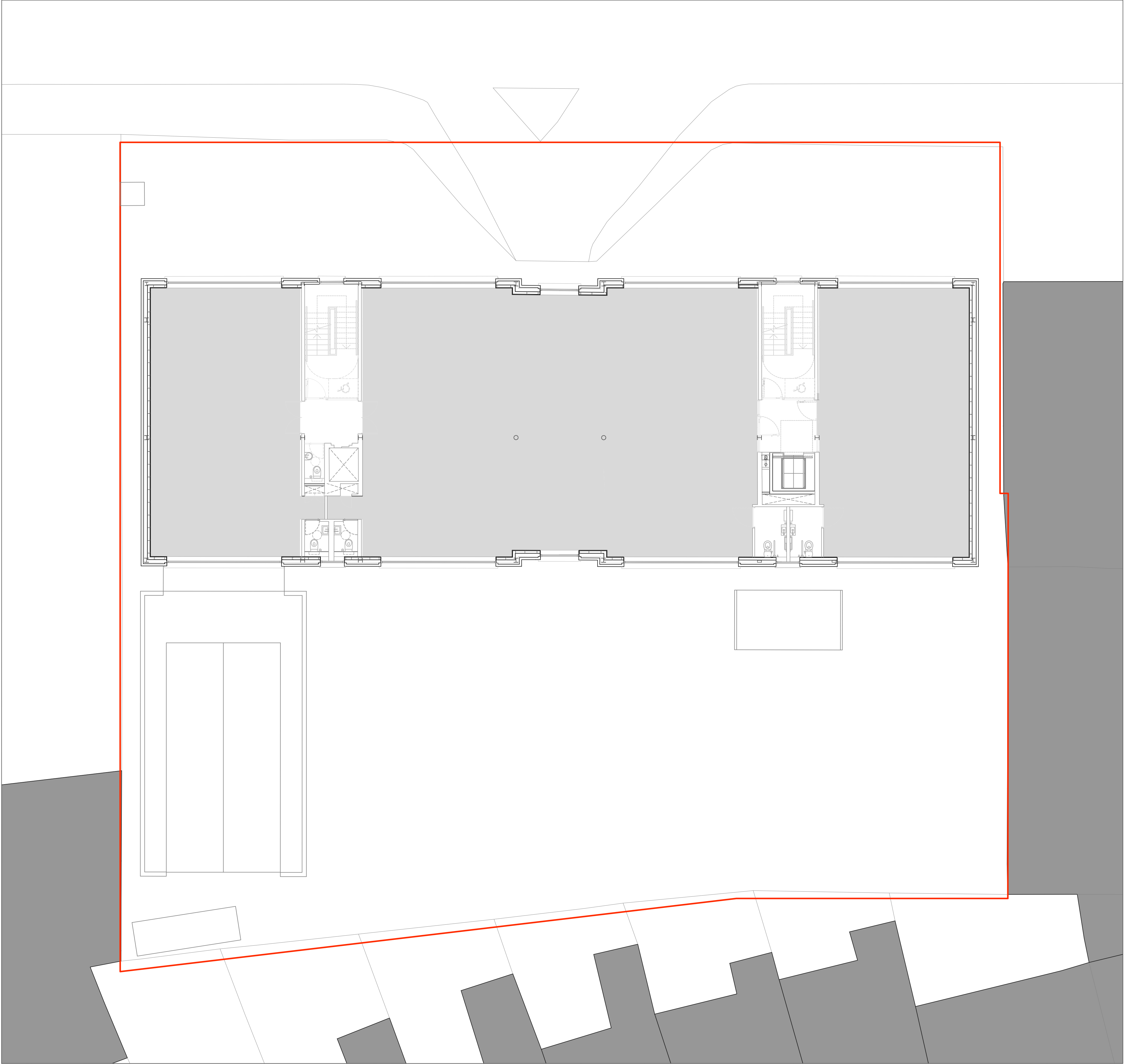
01 Proposed Plan 05-1-103 Third Floor Plan 1:100 @A1
